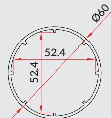
60 Round Pipe (SCW-GF-N103)
