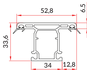
Sliding Sash Mullion (SW-GF-030)
