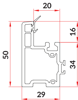
Casement/Sliding Mullion (CW-GF-037)
