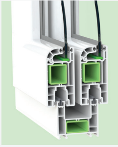
62 Series Sliding System
