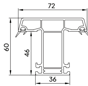
T-Mullion (CW-GF-004)
