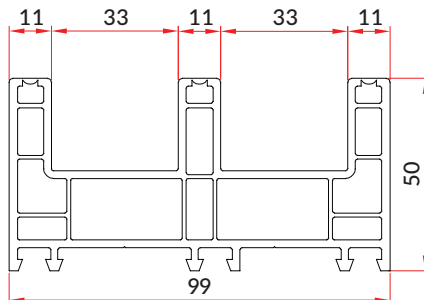
Sliding 3 Track Frame (SW-GF-032)
