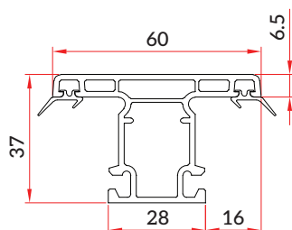
Sash Mullion (SW-GF-016)
