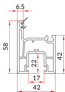
Sliding Window Sash (SW-GF-023)
