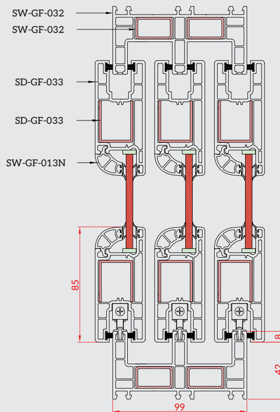
99 Series Sliding System
