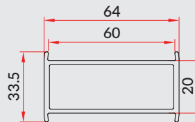
60 Tube Adopter (SCW-GF-N101)
