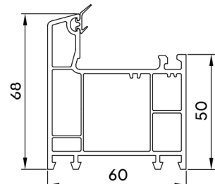
Large Outer Frame (CW-GF-201)
