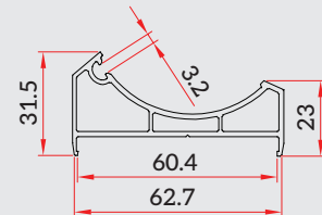
60 Any Angle Bay Corner Adopter (SCW-GF-N102)
