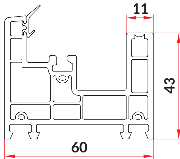
Casement/Sliding Outer Frame (CW-GF-036)
