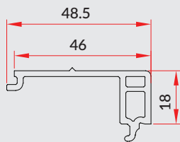
Louver Shutter Bead (SCW-GF-012)
