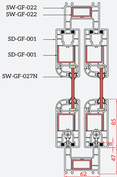
62 Series Sliding System
