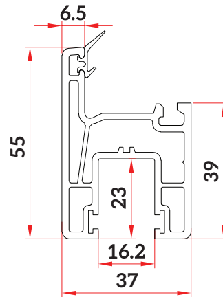
Sliding Window Sash (SW-GF-011)
