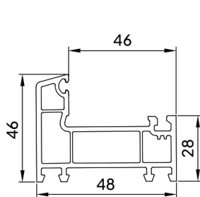
Small Outer Frame (CW-GF-006)
