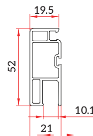
Sliding Window Mesh Sash (SW-GF-012)
