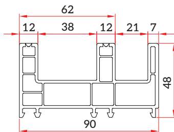
Sliding 2.5 Track Frame with Mesh Rail (SW-GF-020)
