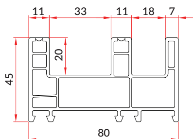
Sliding 2.5 Track Frame (SW-GF-010N)
