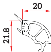
Sliding Glazing Bead (4-6mm) (SW-GF-013N)
