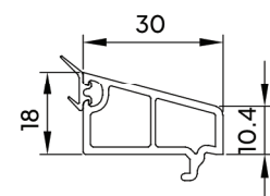
Glazing Bead (8mm) (SCW-GF-016)
