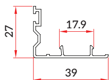
Sliding Window Interlock (SW-GF-014)
