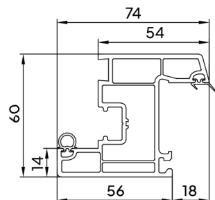
Inward Window Sash (CW-GF-N101)
