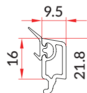
Double Glazing Bead (20mm) (SW-GF-028)
