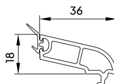
Glazing Bead (4-6mm) (CW-GF-005N)
