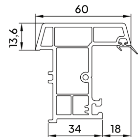
Lap Joint Outer Frame (CW-GF-047)
