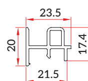
Screen Sash Interlock (SW-GF-018)
