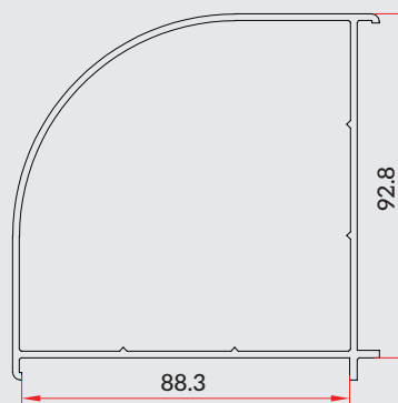
90 Baypole (SCW-GF-009)
