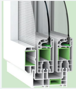
90 Series Sliding System
