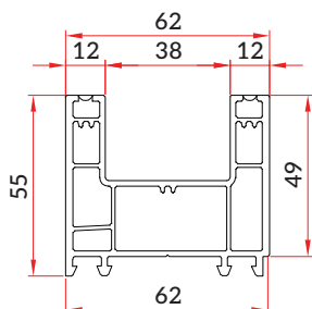
Sliding 2 Track Frame (SW-GF-022)
