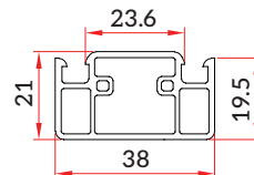
Screen Sash Mullion (SW-GF-017)
