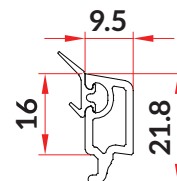
Fixed Glazing Bead (4-6mm) (SW-GF-028)
