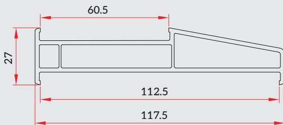
112-60 Coupler (SCW-GF-N107)
