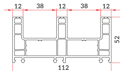
Sliding 3 Track Frame (SW-GF-021)
