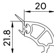
Double Glazing Bead (20mm) (SW-GF-013N)
