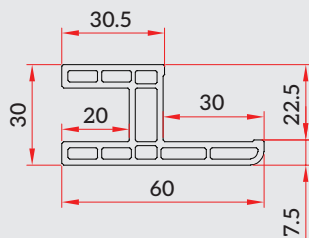
Sliding Screen Sash Frame (SW-GF-035)
