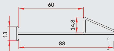
88-60 Coupler (SCW-GF-006)
