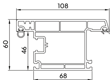
Outward Door Sash (CW-GF-003)
