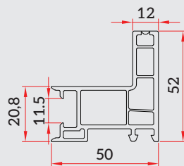
Add On Track (SW-GF-048)
