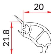
Glazing Bead (10mm) (SW-GF-013N)
