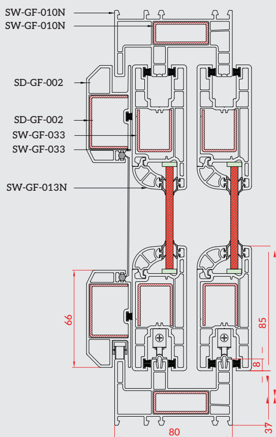
80 Series Sliding System
