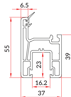
Sliding Window Sash (SW-GF-011)
