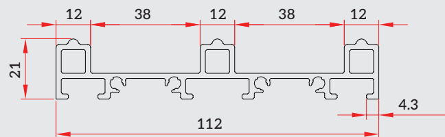
Low Threshold Aluminium (SCW-GF-N109)
