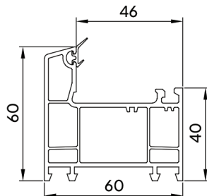
Window Outer Frame (CW-GF-001)
