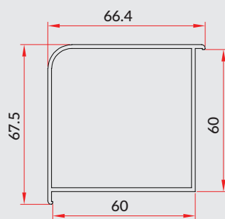
60 Baypole (CW-GF-010)
