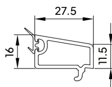
Glazing Bead (12mm) (SCW-GF-015)
