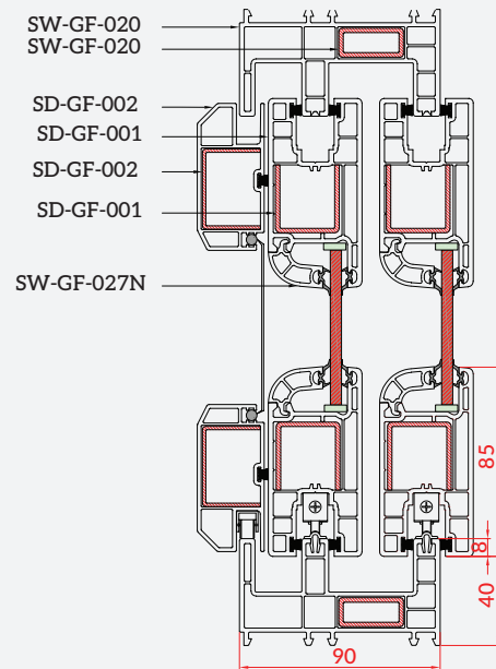
90 Series Sliding System
