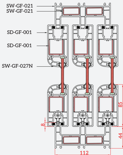
112 Series Sliding System
