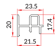
Screen Sash Interlock (SW-GF-018)
