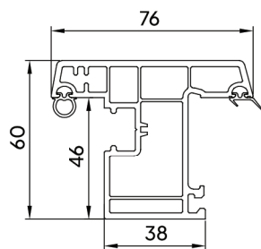
Outward Window Sash (CW-GF-002)
