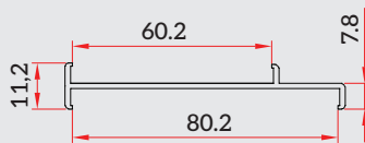
80-60 Coupler (SCW-GF-007)
