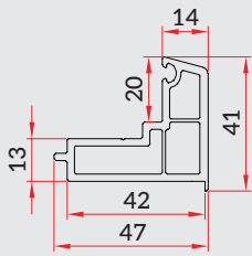
Switch Frame (SCW-GF-N104)
