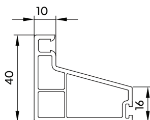
Mesh Sash (CW-GF-007)
